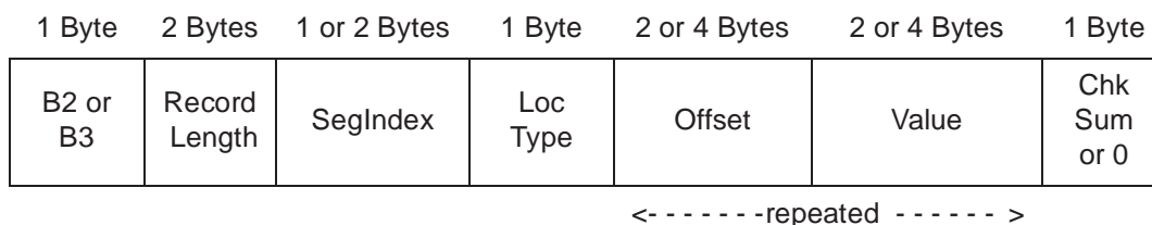
Figure 2-28: BAKPAT Backpatch Record
