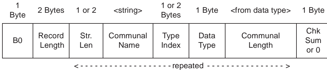
Figure 2-27: COMDEF Communal Names Definition Record
