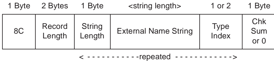
Figure 2-18: EXTDEF External Names Definition Record
