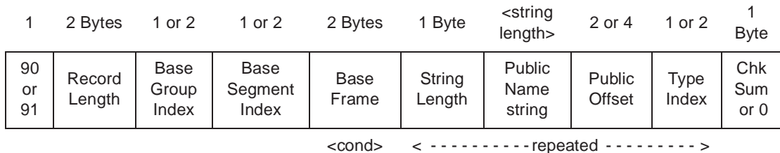
Figure 2-19: PUBDEF Public Names Definition Record
