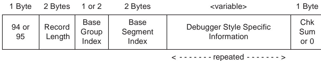
Figure 2-20: LINNUM Line Number Record
