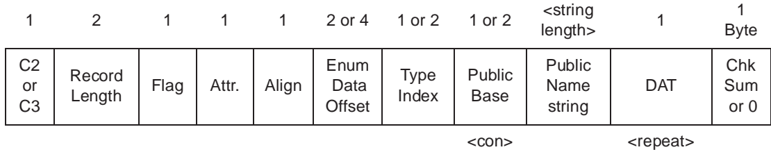
Figure 2-32: COMDAT Initialized Communal Data Record
